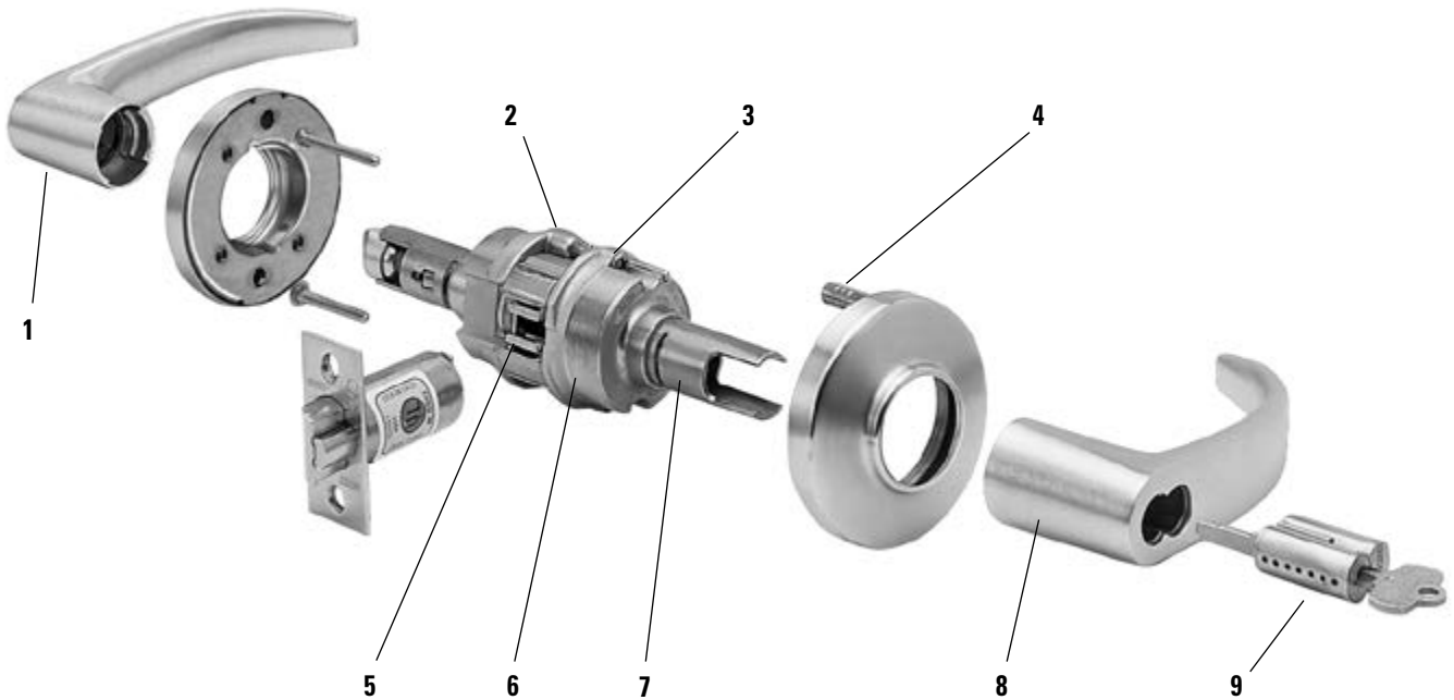
9K – EXPLODED
