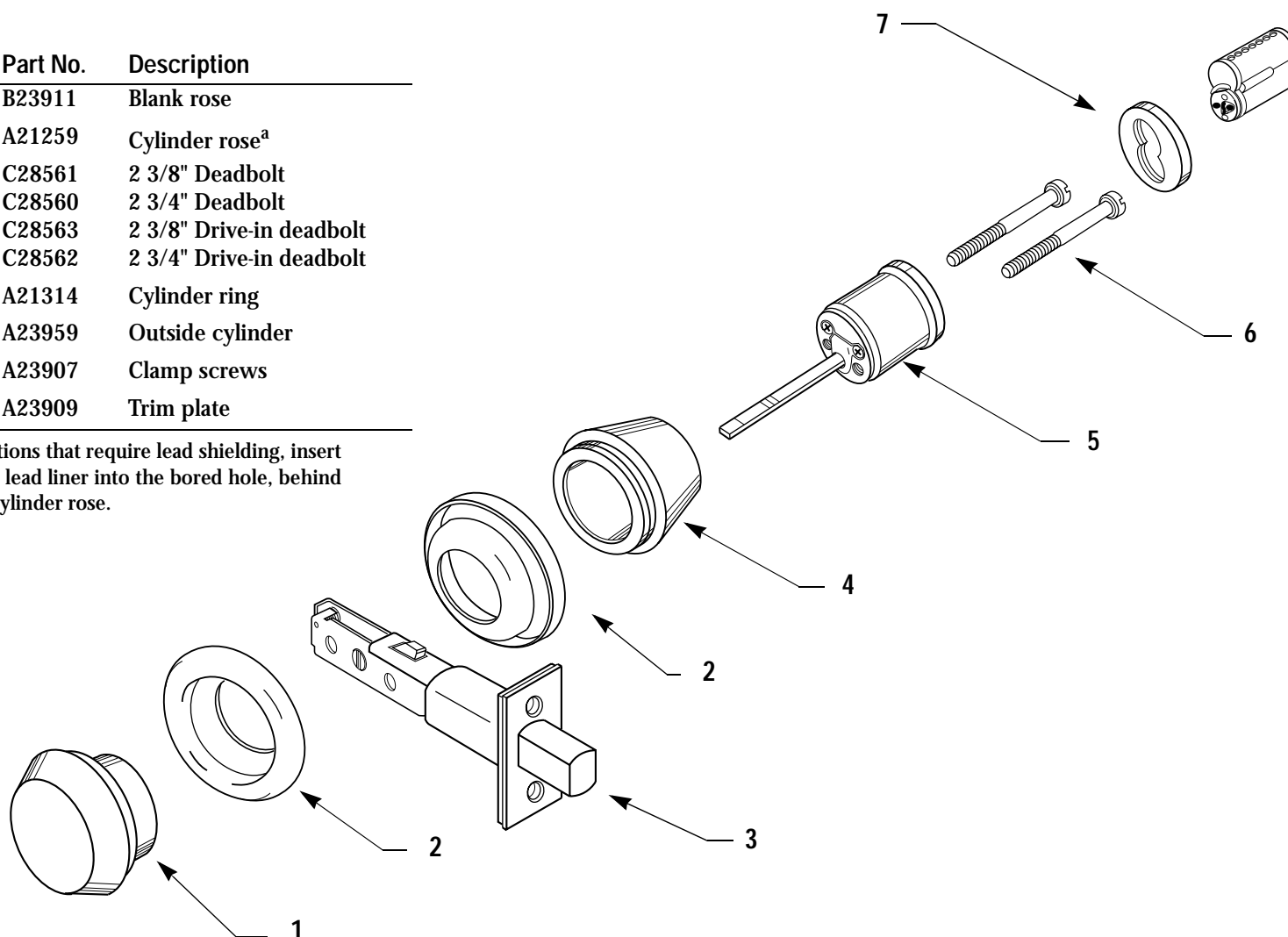
Figure 3.4 L function with concealed screws exploded diagram—deadbolt operated from one side only
