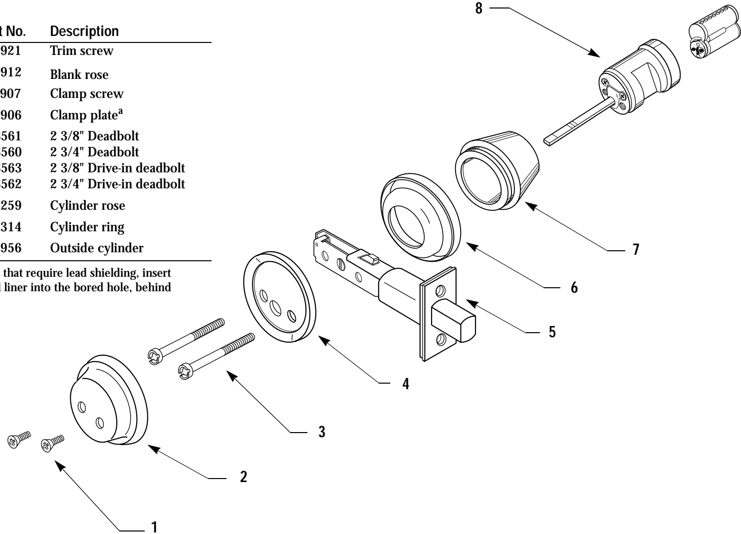
Figure 3.3 L function exploded diagram—deadbolt operated from one side only
